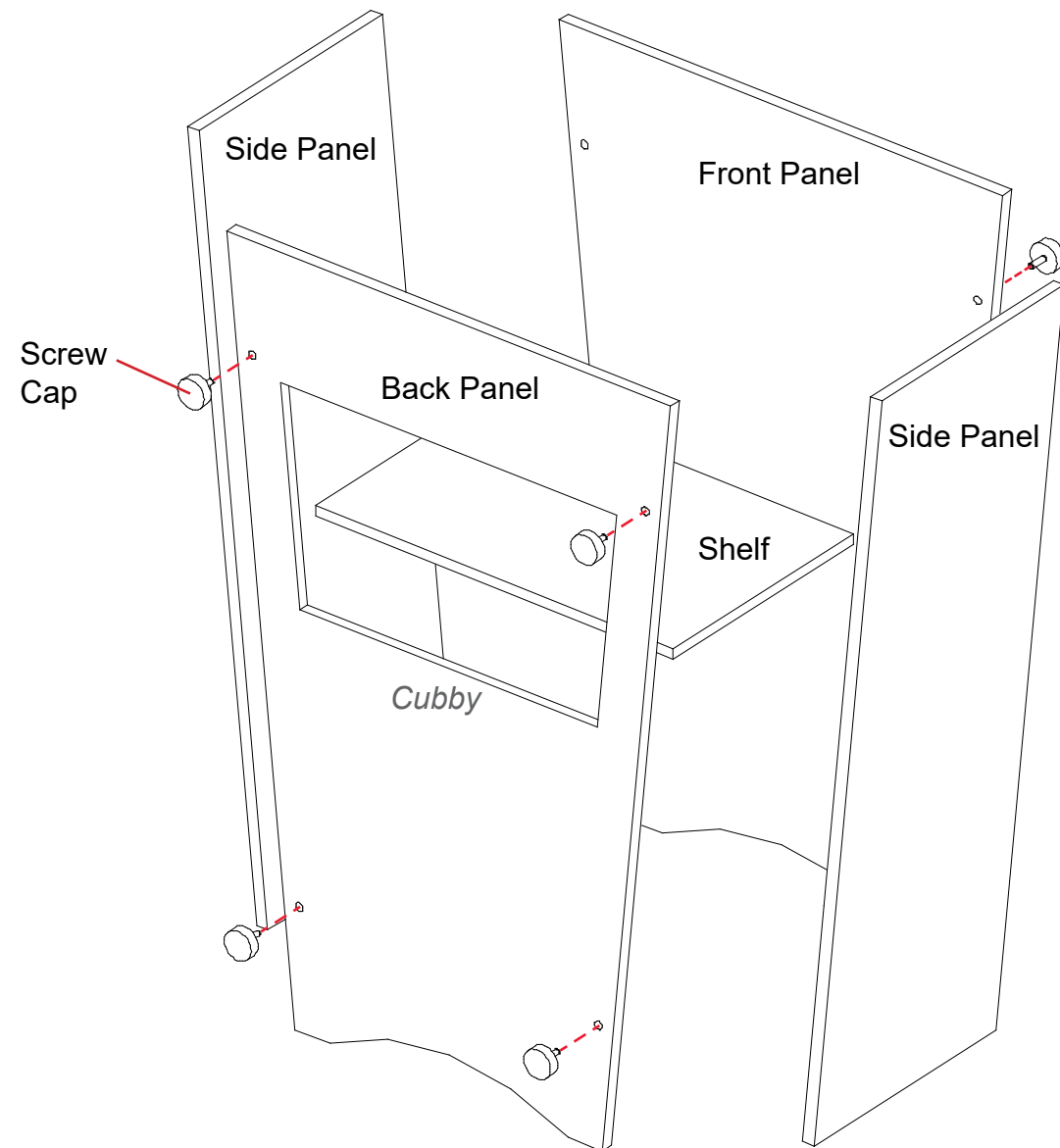
Pedestal Base Assembly
